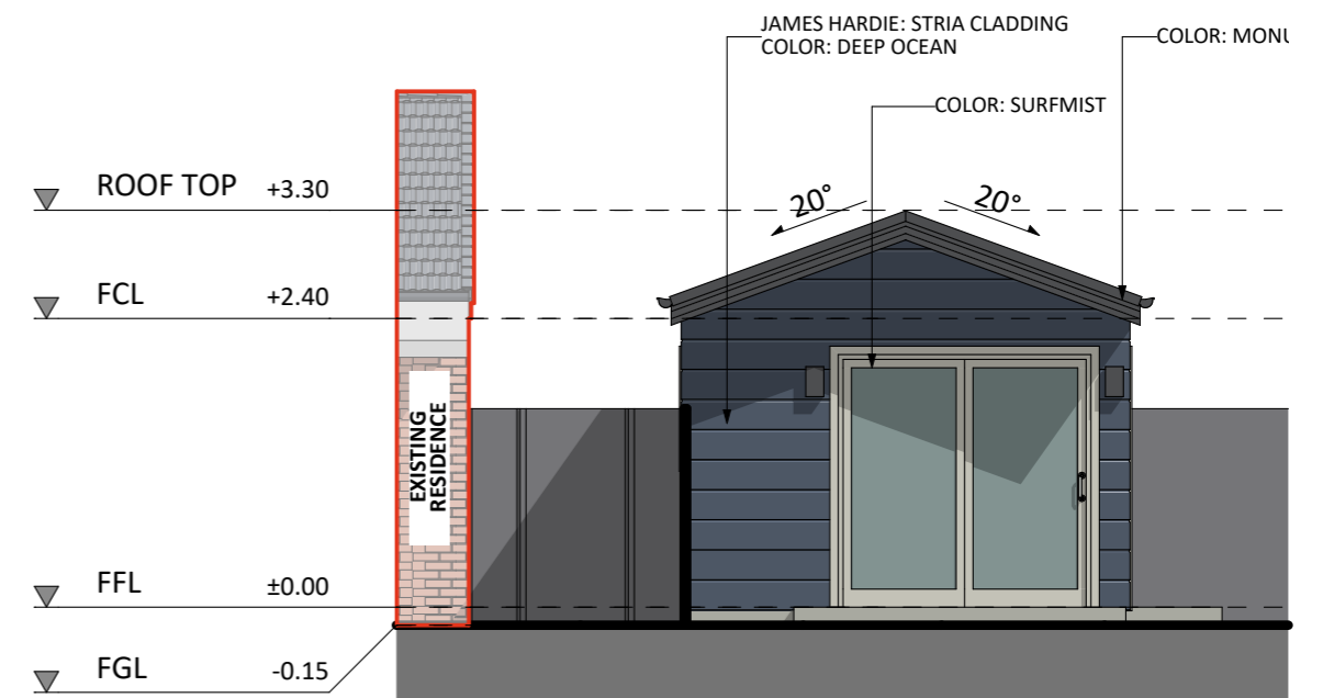
NORTH-WEST ELEVATION
