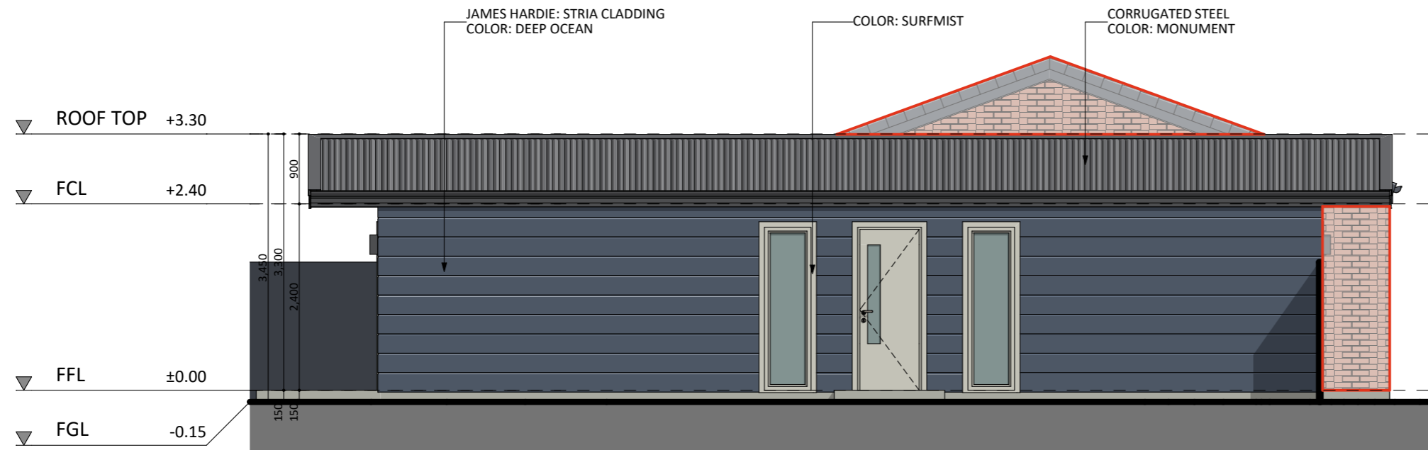
SOUTH-WEST ELEVATION
